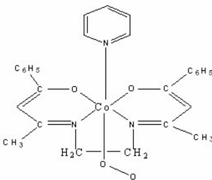
Co(acacen) complex
